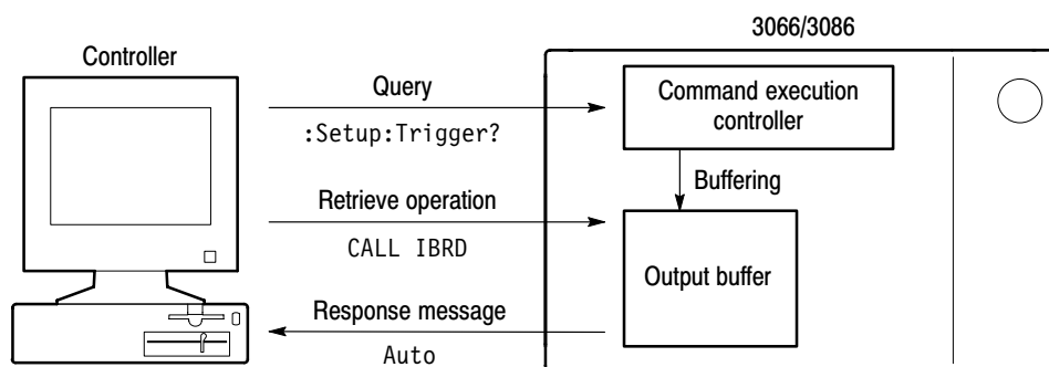
Figure 2-12: Retrieving response message
