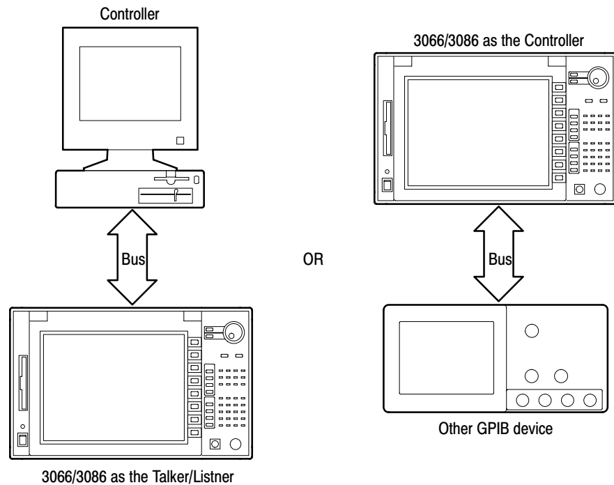
Figure 1-6: GPIB connection
